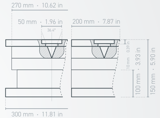
Mold Set
