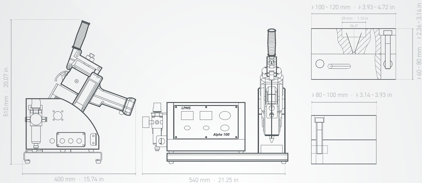
Machine
